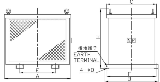
図-4 ・TTSH-150KLG~TTSH-200KLG
